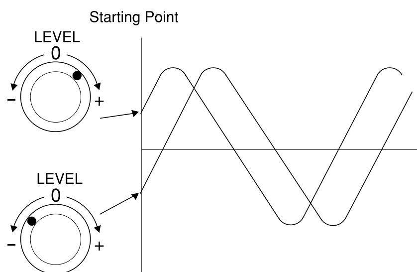
FIGURE 2-5. TRIGGER LEVEL CONTROL
