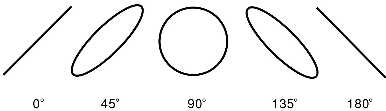
(b) LISSAJOUS PATTERNS OF VARIOUS PHASE ANGLES
